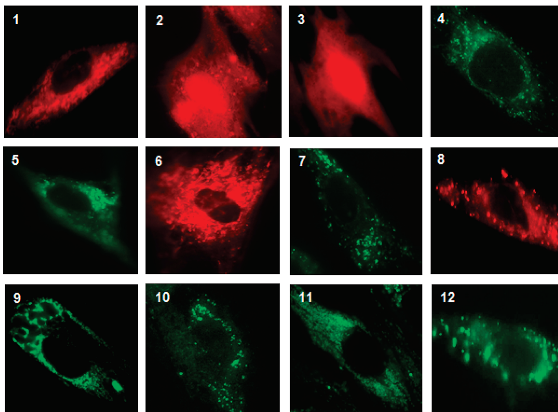
Figure 1. Fluorescence microscopy images for probes 1–12. Cells were incubated with 1 \mu M fluorophore for 2 h and then washed with PBS to remove any unincorporated fluorophores. Images were taken using a Nikon Eclipse 80i microscope equipped for epifluorescence using filter sets as described in the Experimental Section. A 60 \times objective was used, and the microscope parameters, including fluorescence intensity and exposure, were optimized for each fluorophore.
