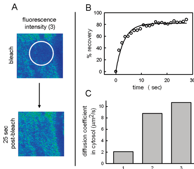
Figure 3. Results of FRAP assays. (A) Fluorescence images immediately following photobleaching (top) and 25 s post-bleach period (bottom) for probe 3 . (B) Correlation plot of % fluorescence recovery as a function of time for probe 3 . (C) Diffusion coefficient values for probes 1–3 . The diffusion coefficient is obtained by dividing the area of the photobleached region by the half-life for fluorescence recovery in that region. The diffusion coefficients for probes 4–12 are not included on the graph and were all less than 0.5 \mu\text{m}^2/\text{s} .
