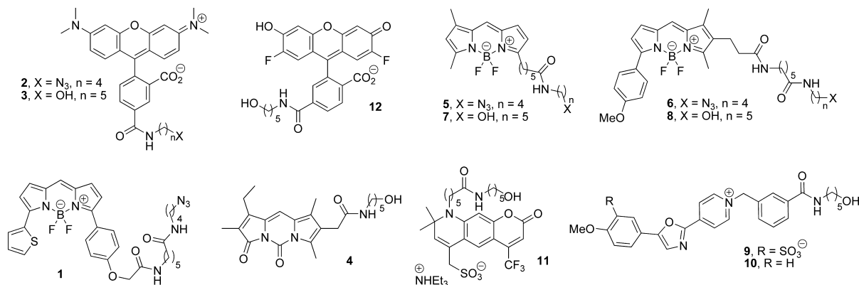
Chart 1. Structures of Fluorescent Probes 1–12
