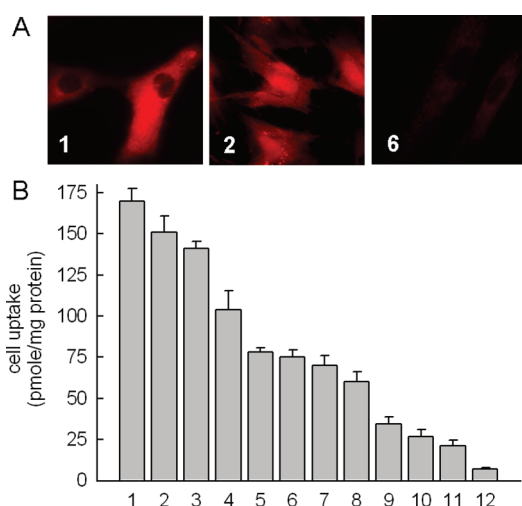
Figure 2. (A) Qualitative comparison of fluorescence microscopy images of 1, 2, and 6. Fluorescence images were taken using conditions as described in the Experimental Section. (B) Quantitative comparison of cellular uptake for 1–12. Cells were treated with the test compound to a final concentration of 2 \mu M for 2 h before evaluation. Cellular uptake of each compound was determined and normalized to protein concentration in the sample.
