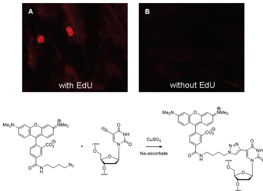
Figure 4. Click chemistry within cells. The modified thymidine derivative 5-ethynyl-2'-deoxyuridine (EdU, Berry & Associates) was incorporated into DNA of normal human fibroblast cells according to the method described in ref 38. Fibroblast cells which were not treated with EdU were used as a negative control. Cells were then preincubated with TAMRA-N 3 ( 3 , 1 \mu M) for 3 h before treatment with CuSO 4 (0.5 mM) and ascorbic acid (100 mM) for 15 min. Following that, cells were quickly washed several times to remove any unbound fluorophore. Live cell images of cells which had been modified with EdU (panel A) showed a large degree of nuclear staining, indicating covalent attachment of the fluorescent probe with DNA. This was not seen with control cells that did not incorporate alkynes (panel B).
